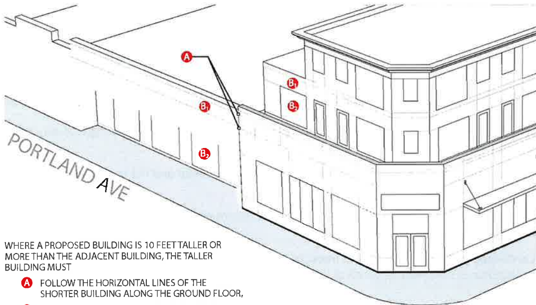
FIGURE 4: BUILDING FORM
